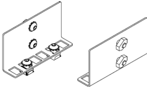
AVALL rack mount brackets (Max 2U)
